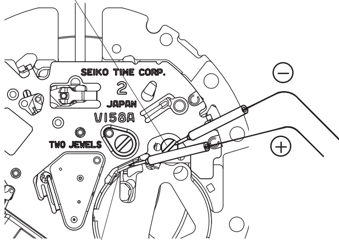
BATTERY CONNECTION (+)
